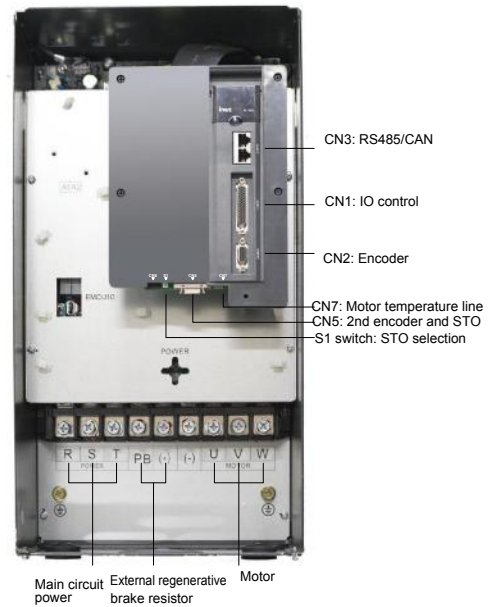
Frame size G
