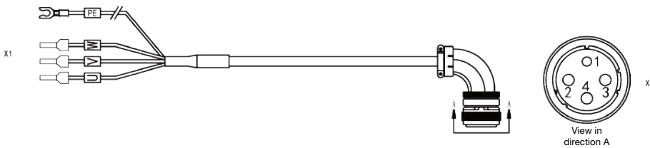
Power cable for 180 base (YD32 plug)
