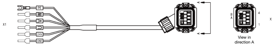
Power cable for 130 base (YD28 plug)
